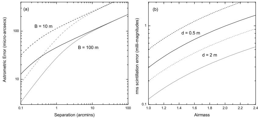
Figure 2. (a) Astrometric error versus angular separation for a 10 m (black) and 100 m (grey) baseline interferometer with a 1 hour integration at Dome C (solid) compared with Mauna Kea (dashes) (b) Scintillation-limited photometric precision as a function of airmass for 0.5 m (black) and 2 m (grey) telescopes at Dome C (solid) compared to Mauna Kea (dashes).
