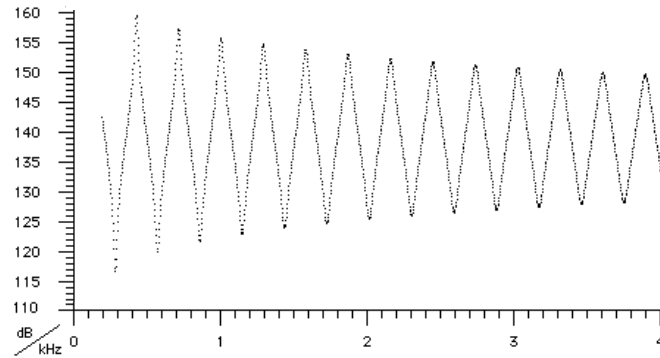
Figure 3. Z(f) for an open, stainless steel cylinder of length 596.7 mm and diameter 7.8 mm.
