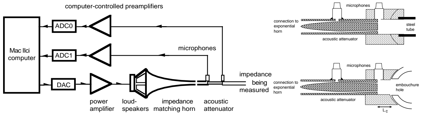
Figure 2. The impedance spectrometer (a) and the configuration for calibration (b) and for measurement (c). The figure is not to scale.
