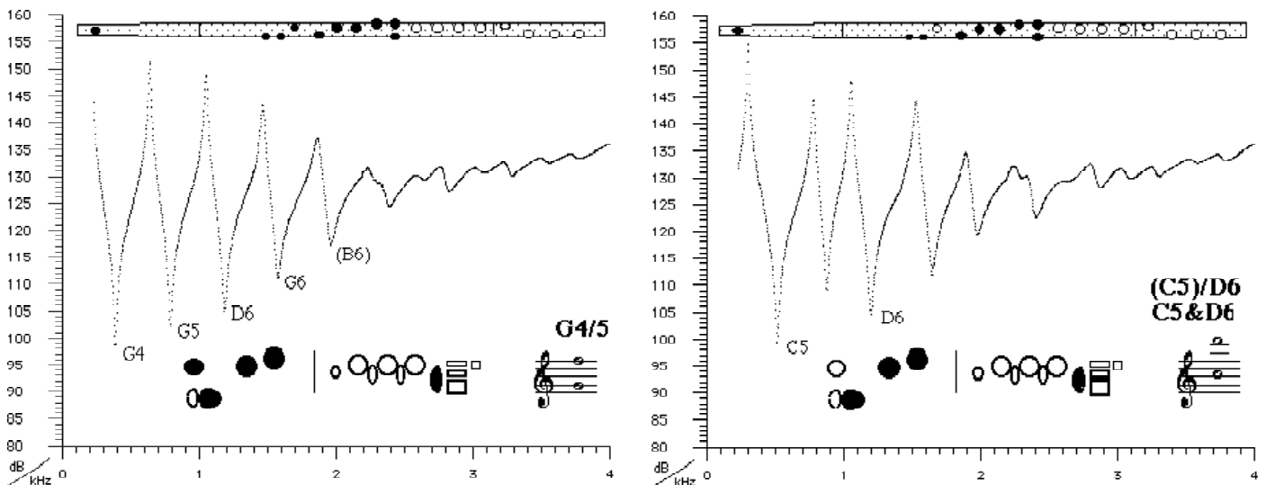
Figure 7. The input impedance Z(f) for the cases described in Figure 6.
