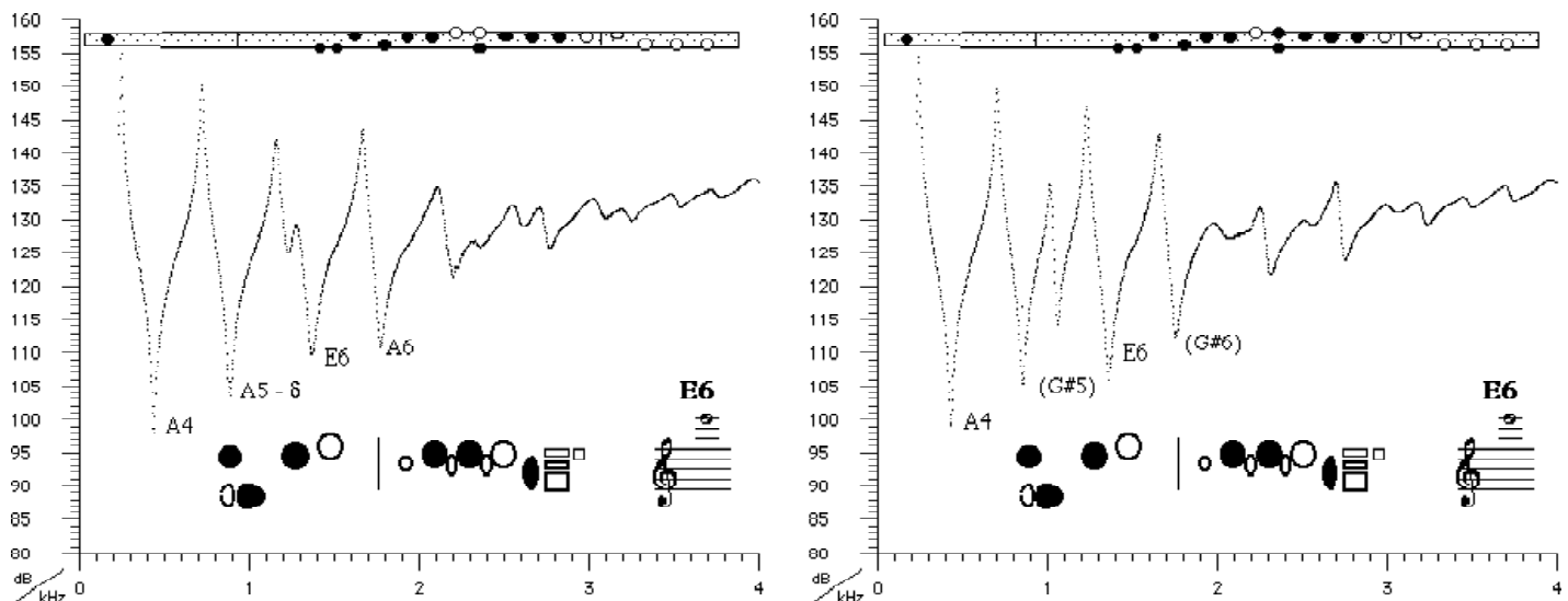
Figure 8. Impedance spectra for the note E6, without (left) and with a 'split E mechanism' (right)
