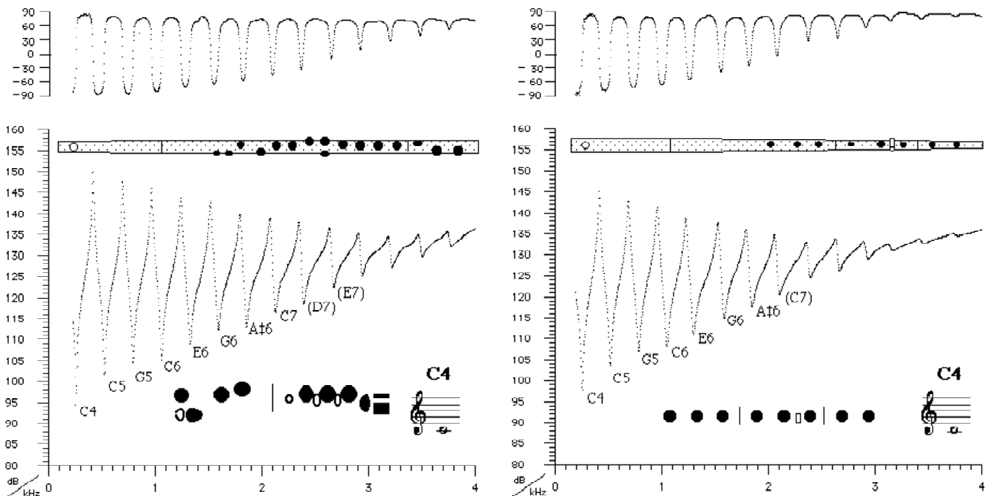
Figure 4. Z(f) (phase in degrees and magnitude in dB) for a modern flute (left) and a classical flute (right) for the note C4.
