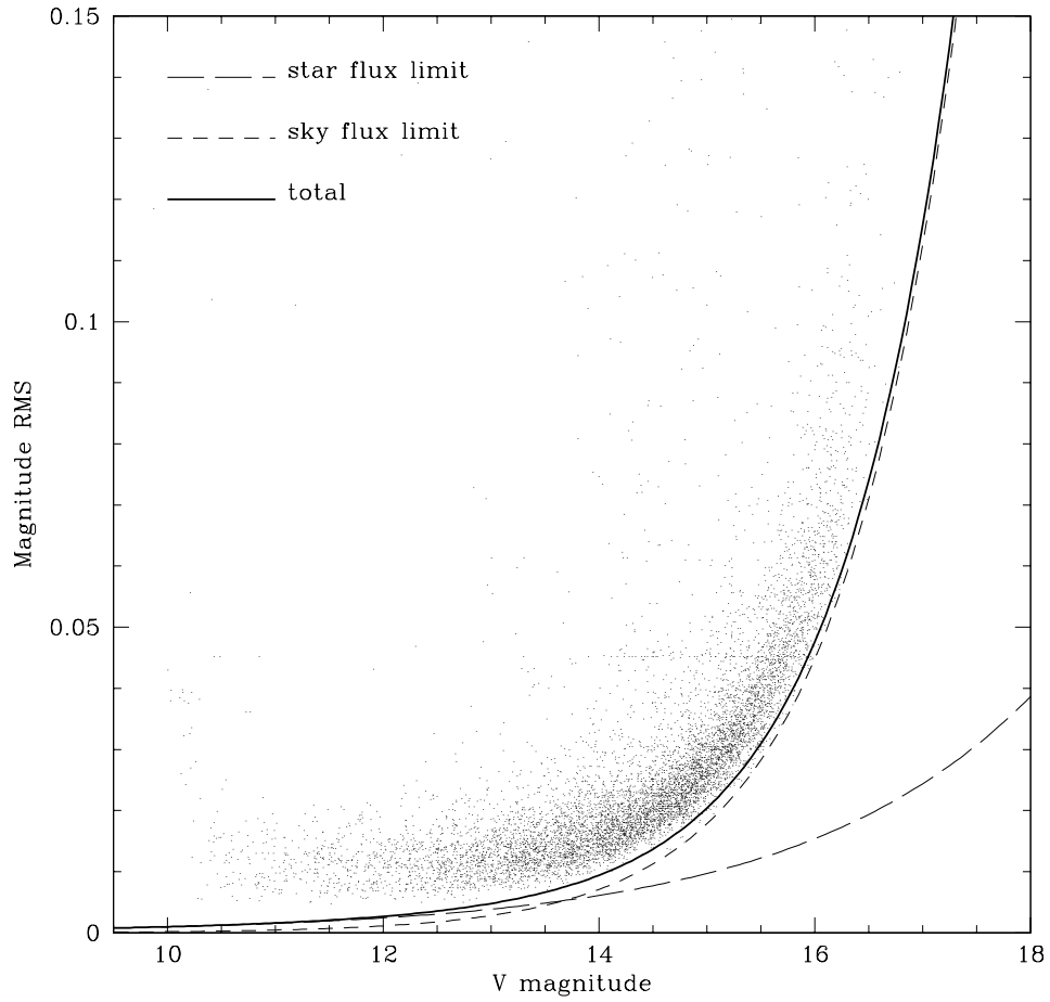
Figure 1. Photometric precision for a series of 150 second exposures taken with the APT. The field is centered on the open cluster NGC6633, close to the Galactic plane. The limits due to photon shot noise in the star and sky flux are shown. Readout noise is negligible. Systematic errors limit the precision for bright stars. Stars brighter than V \sim 10.5 are saturated.
