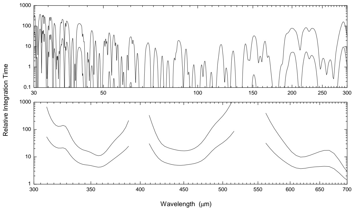
Fig. 10.— The ratio of point-source integration times for a 2.4 m airborne telescope (in the top panel) and a 15 m Chajnantor Plateau telescope (bottom panel) to a 12 m Antarctic telescope. In each panel both Dome C (lower curve) and Dome A (upper curve) sites are considered. Values are only shown for wavelengths at which the Chajnantor Plateau transmission is greater than 10%.
