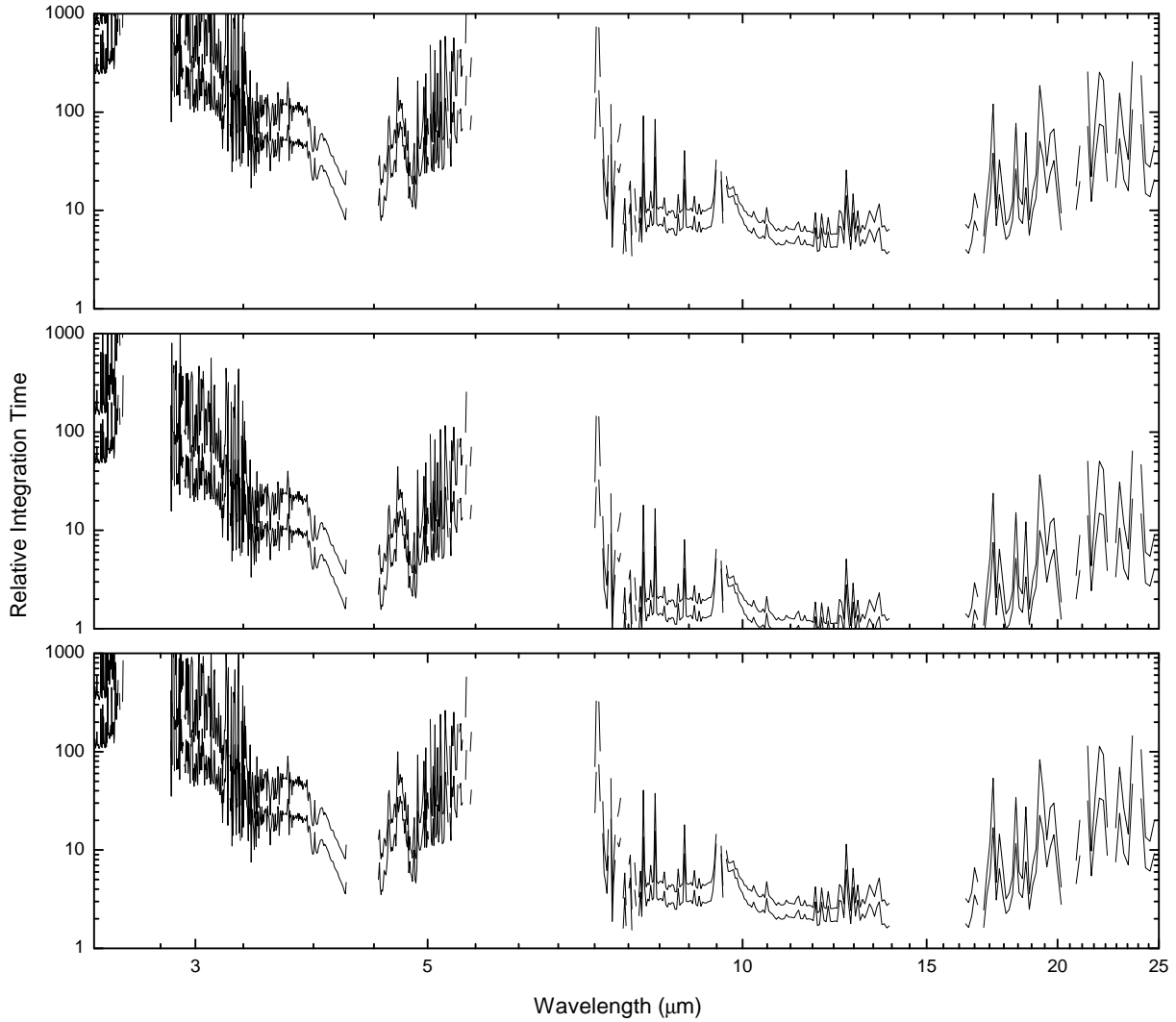
Fig. 9.— The ratio of point-source integration times for a 30 m Mauna Kea telescope with a 30 m Antarctic telescope (top panel), and a 20 m Antarctic telescope (bottom two panels). Each telescope is seeing limited (with the same seeing size) for the middle panel. Each telescope is diffraction limited in the bottom panel. In each panel both Dome C (lower curve) and Dome A (upper curve) sites are considered. Values are only shown for wavelengths at which the Mauna Kea transmission is greater than 10%.
