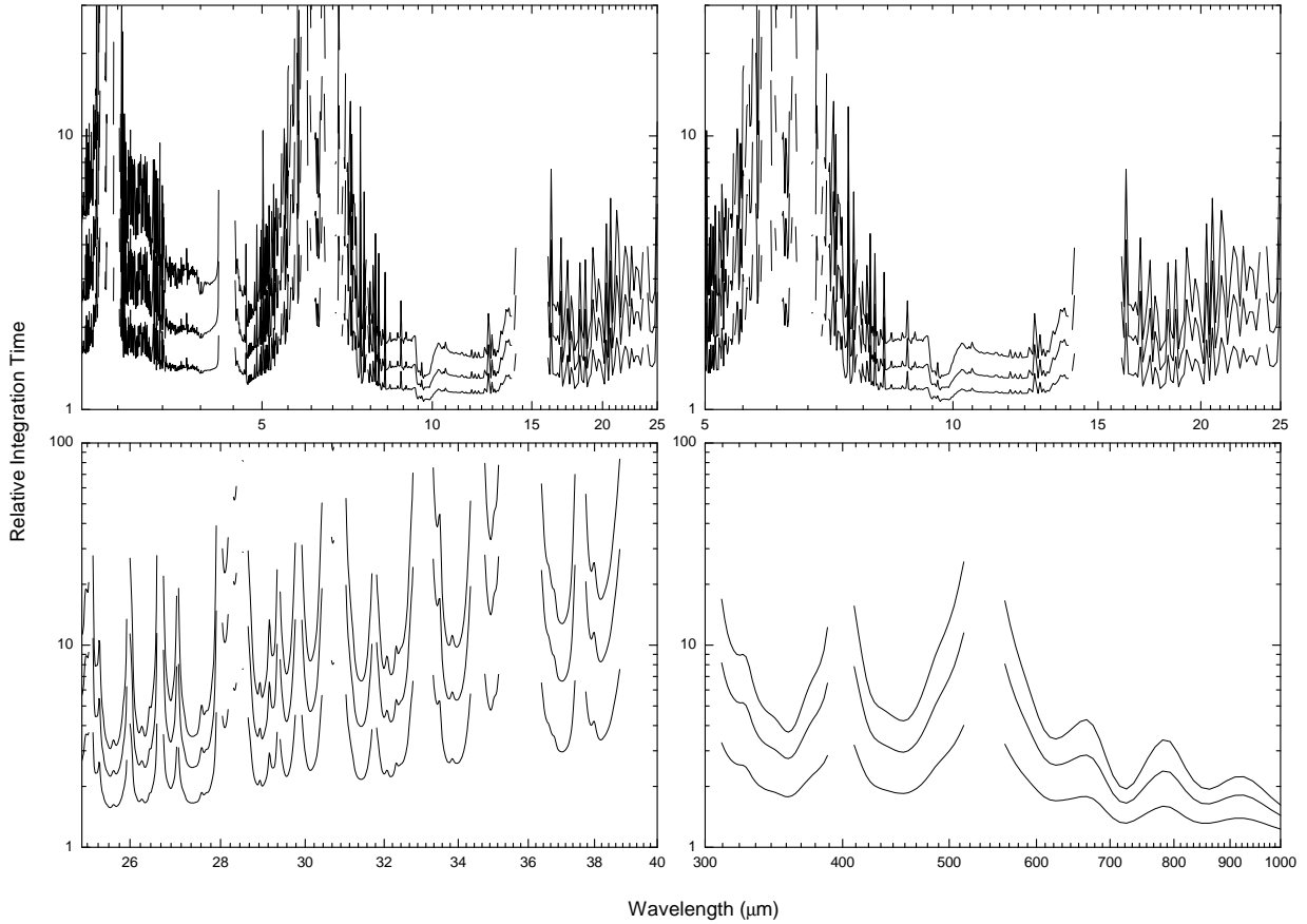
Fig. 8.— Ratio of integration times from the near-infrared to sub-millimetre for a South Pole telescope compared with a Dome C (bottom curve), Dome F (middle curve), and Dome A (top curve) telescope. Each telescope is assumed diffraction-limited and equivalent in all aspects. Values are only shown for wavelengths at which the South Pole transmission is greater than 10%.
