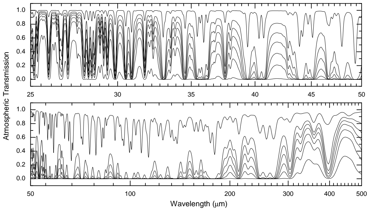
Fig. 7.— Atmospheric transmission in the far infrared/submillimetre. The plot shows, in order of increasing transmission at any wavelength, Chajnantor Plateau, South Pole, Dome C, Dome Fuji, Dome A (average conditions), Dome A (good conditions), and SOFIA. The pwv content for each model atmosphere is 1000, 250, 175, 105, 60, 30, and 10 \mu\text{m} respectively.
