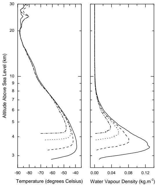
Fig. 1.— Temperature profiles (left plot) and water vapour density profiles (right plot) for the model atmospheres. The South Pole (solid line) and Dome Fuji (dot line) profiles represent averages from radiosonde balloon launches. The Dome C (dash line) and Dome A (dash-dot line) profiles are interpolated/extrapolated from these (see text).
