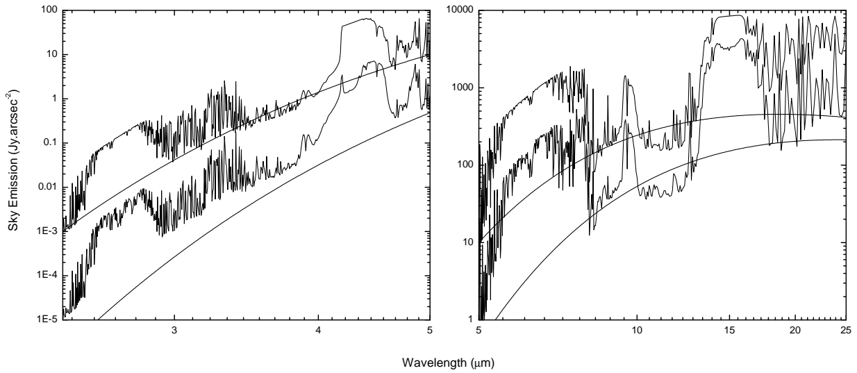
Fig. 3.— Model winter-time sky emission in the near and mid-infrared for Mauna Kea (top curve) and South Pole (bottom curve). The emission from a 5% emissive telescope at ground temperatures of -60^{\circ} C and 0^{\circ} C are also shown.
