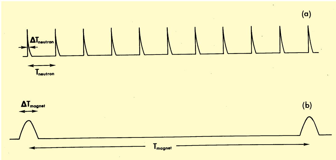
Figure 3. Schematic figure showing the pulse-lengths \Delta T and periods T of (a) the pulsed spallation neutron source and (b) the pulsed magnet. In our proposal, \Delta T_{\text{neutron}} = 25 - 100 \mu\text{s} , \Delta T_{\text{magnet}} = 3 \text{ ms} , T_{\text{neutron}} = 50 \text{ ms} , and T_{\text{magnet}} = 0.5 \text{ s} .
